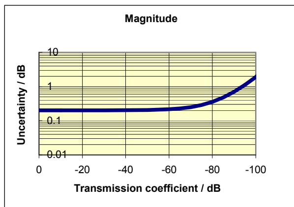
Typical accuracy of transmission magnitude and transmission phase measurements of the R&S®ZVA40 in the frequency range 24 GHz to 40 GHz.
