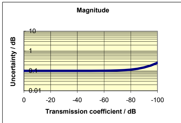
Typical accuracy of transmission magnitude and transmission phase measurements of the R&S®ZVA50 and R&S®ZVA67 in the frequency range 700 MHz to 24 GHz.
