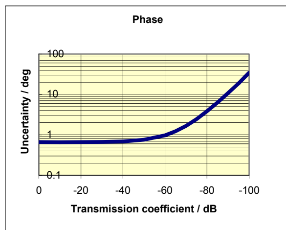
Typical accuracy of transmission magnitude and transmission phase measurements of the R&S®ZVA24 in the frequency range 10 MHz to 700 MHz.
