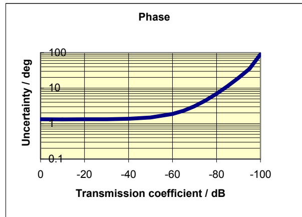
Typical accuracy of transmission magnitude and transmission phase measurements of the R&S®ZVA50 and R&S®ZVA67 in the frequency range 10 MHz to 700 MHz.
