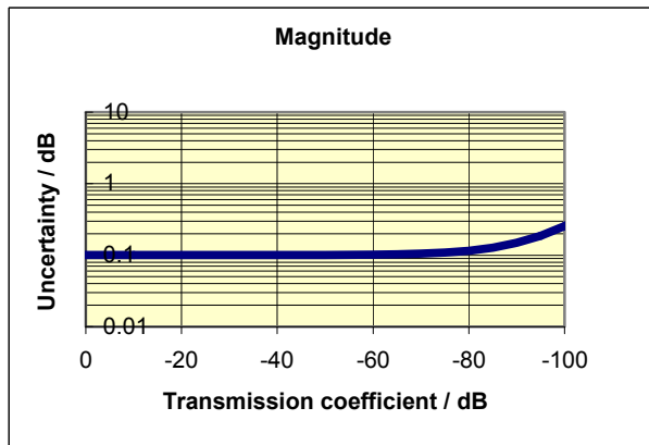
Typical accuracy of transmission magnitude and transmission phase measurements of the R&S®ZVA40 in the frequency range 700 MHz to 24 GHz.
