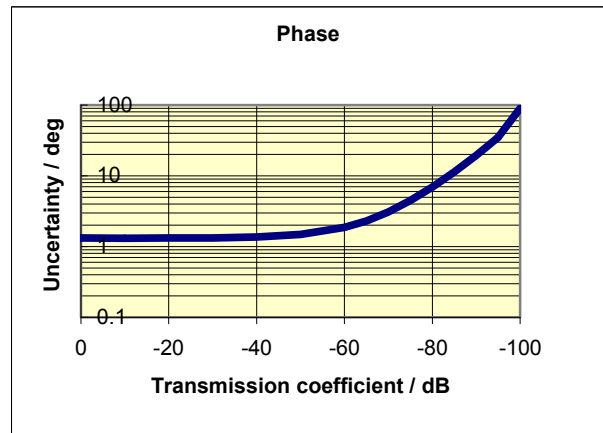
Typical accuracy of transmission magnitude and transmission phase measurements of the R&S®ZVA40 in the frequency range 10 MHz to 700 MHz.
