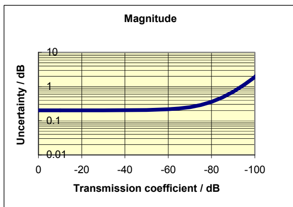
Typical accuracy of transmission magnitude and transmission phase measurements of the R&S®ZVA50 and R&S®ZVA67 in the frequency range 24 GHz to 50 GHz.
