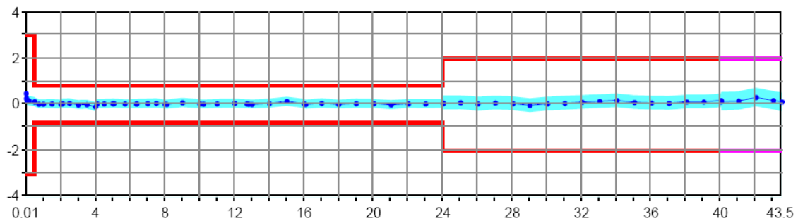
Output power accuracy in dB versus frequency in GHz of the R&S®ZVA40.
