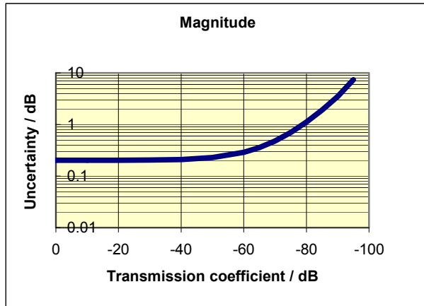
Typical accuracy of transmission magnitude and transmission phase measurements of the R&S®ZVA50 and R&S®ZVA67 in the frequency range 10 MHz to 700 MHz.
