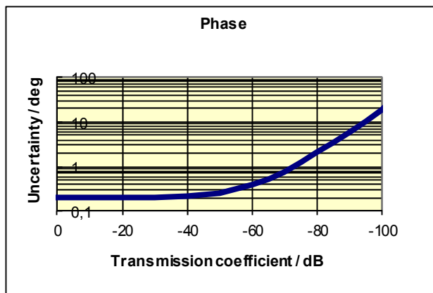
Typical accuracy of transmission magnitude and transmission phase measurements of the R&S®ZVA8 in the frequency range 300 kHz to 50 MHz.
