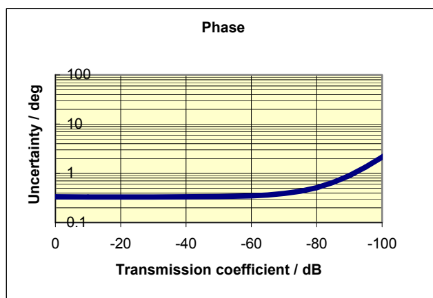
Typical accuracy of transmission magnitude and transmission phase measurements of the R&S®ZVA8 in the frequency range 50 MHz to 8 GHz.
