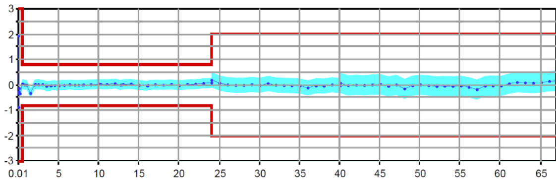
Output power accuracy in dB versus frequency in GHz of the R&S®ZVA67.
