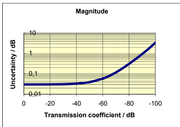
Typical accuracy of transmission magnitude and transmission phase measurements of the R&S®ZVA8 in the frequency range 300 kHz to 50 MHz.
