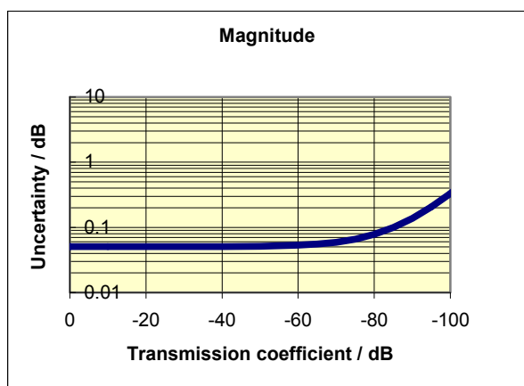
Typical accuracy of transmission magnitude and transmission phase measurements of the R&S®ZVA8 in the frequency range 50 MHz to 8 GHz.
