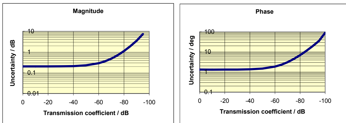
Typical accuracy of transmission magnitude and transmission phase measurements of the R&S®ZVA67 in the frequency range 50 GHz to 67 GHz.
