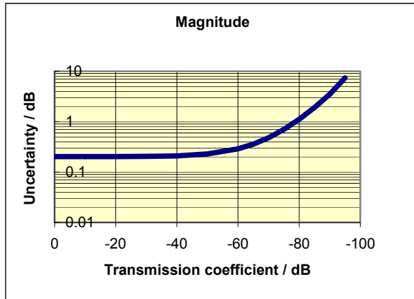
Typical accuracy of transmission magnitude and transmission phase measurements of the R&S®ZVA40 in the frequency range 10 MHz to 700 MHz.
