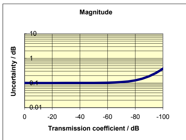
Typical accuracy of transmission magnitude and transmission phase measurements of the R&S®ZVA24 in the frequency range 700 MHz to 24 GHz.
