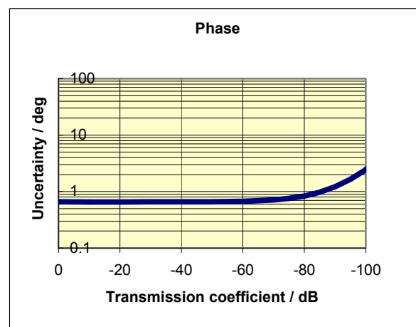
Typical accuracy of transmission magnitude and transmission phase measurements of the R&S®ZVA24 in the frequency range 700 MHz to 24 GHz.
