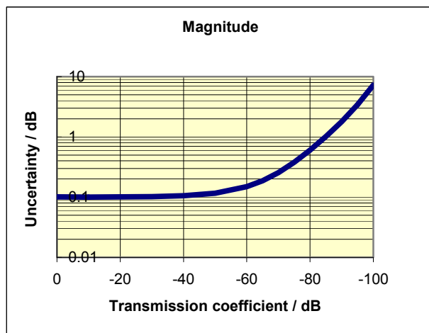
Typical accuracy of transmission magnitude and transmission phase measurements of the R&S®ZVA24 in the frequency range 10 MHz to 700 MHz.
